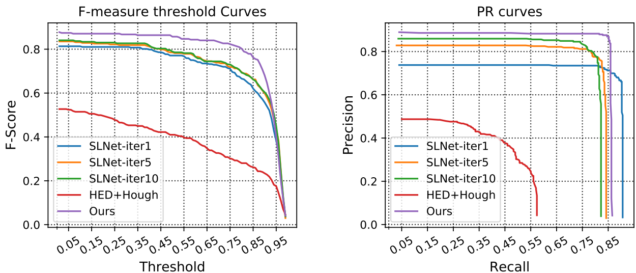
Fig. 12. Left: F-measure under various thresholds. Right: The precision-recall curve. Our method outperforms SLNet [11] and classical Hough transform [25] with a considerable margin. Moreover, even with 10 rounds of location refinement, SLNet still presents inferior performance.
