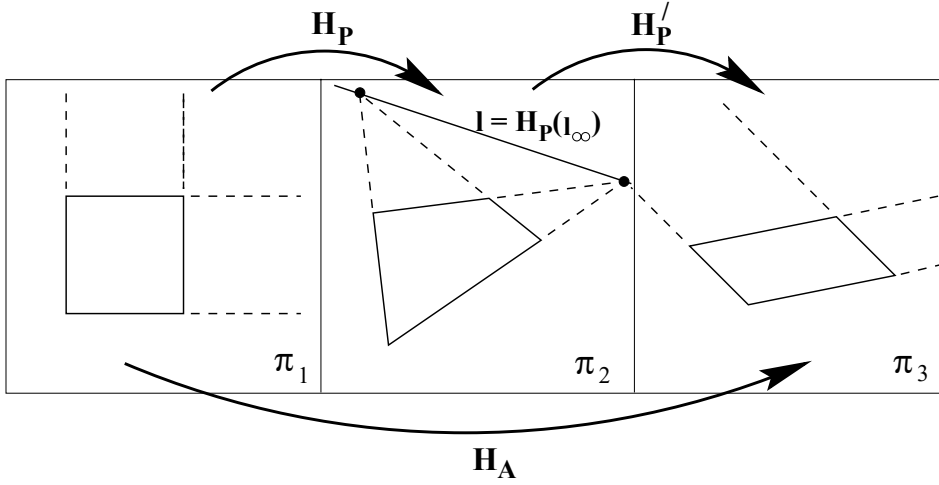
Fig. 2.12. Affine rectification. A projective transformation maps \mathbf{l}_\infty from (0, 0, 1)^\top on a Euclidean plane \pi_1 to a finite line \mathbf{l} on the plane \pi_2 . If a projective transformation is constructed such that \mathbf{l} is mapped back to (0, 0, 1)^\top then from result 2.17 the transformation between the first and third planes must be an affine transformation since the canonical position of \mathbf{l}_\infty is preserved. This means that affine properties of the first plane can be measured from the third, i.e. the third plane is within an affinity of the first.
